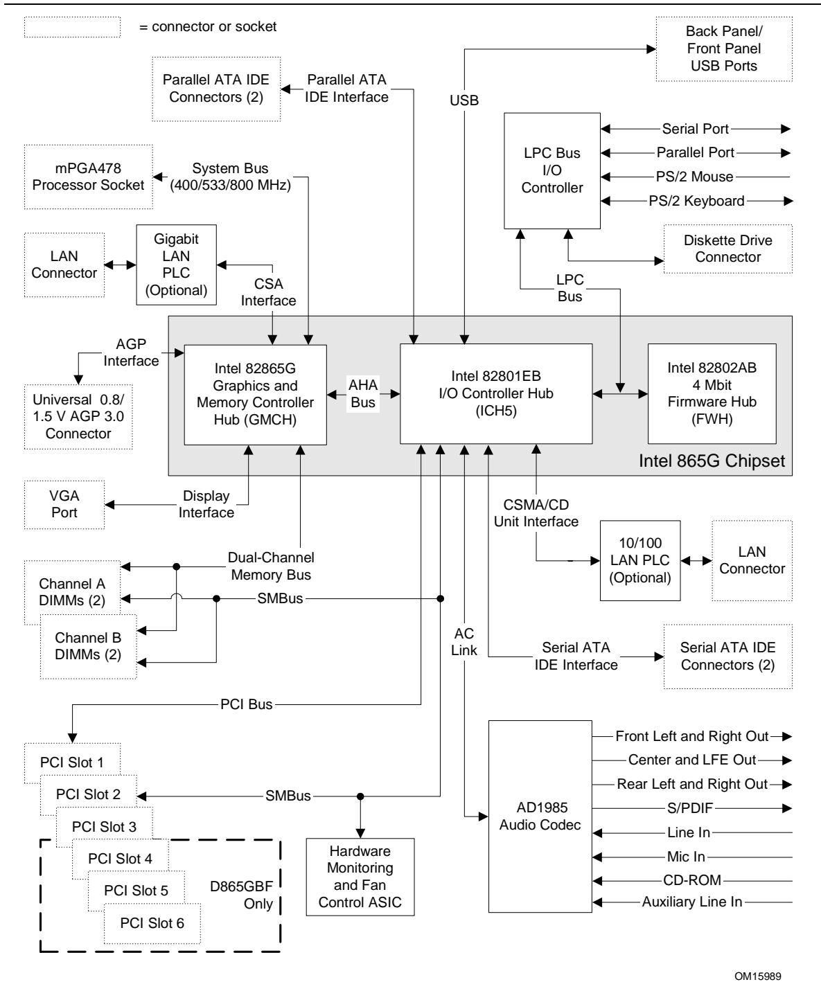
Figure 3. Block Diagram
